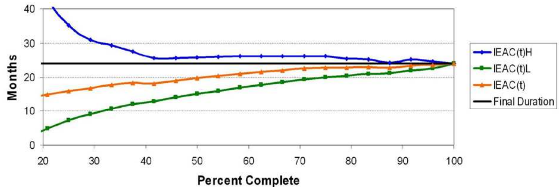
Figure 2. Statistical Forecasting
